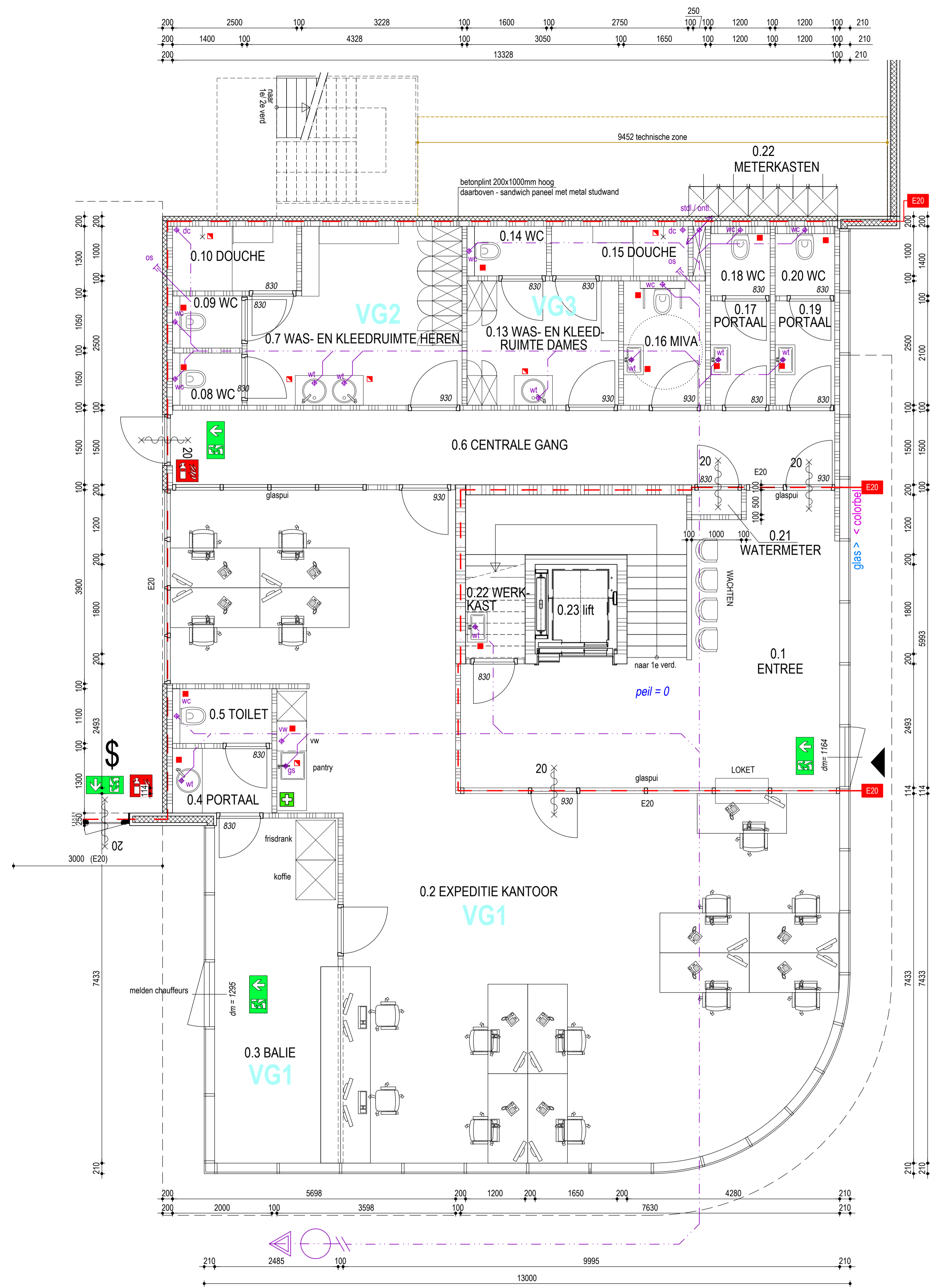
BEGANE GROND Peil = 0
